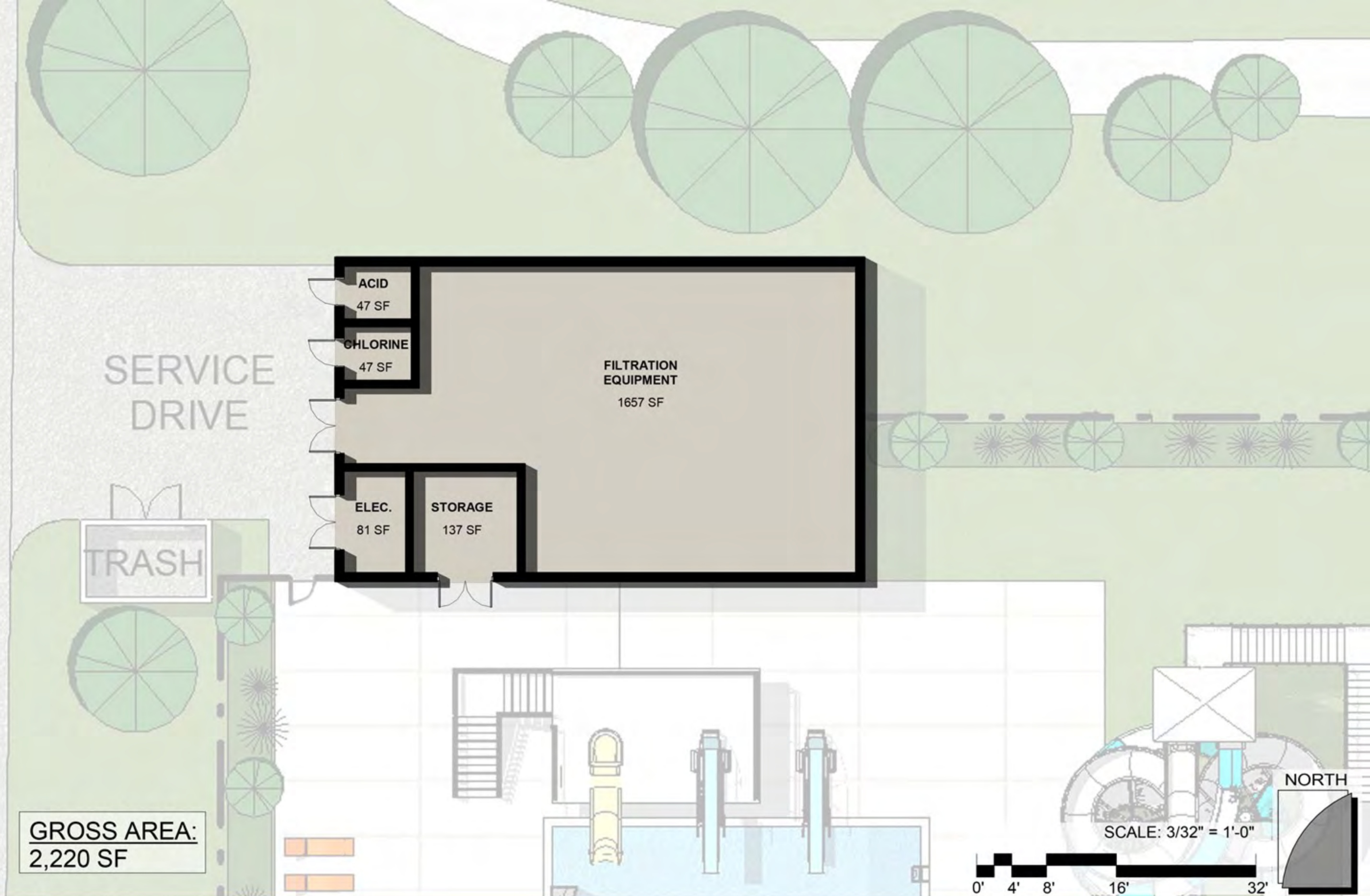
FILTER BUILDING PLAN
